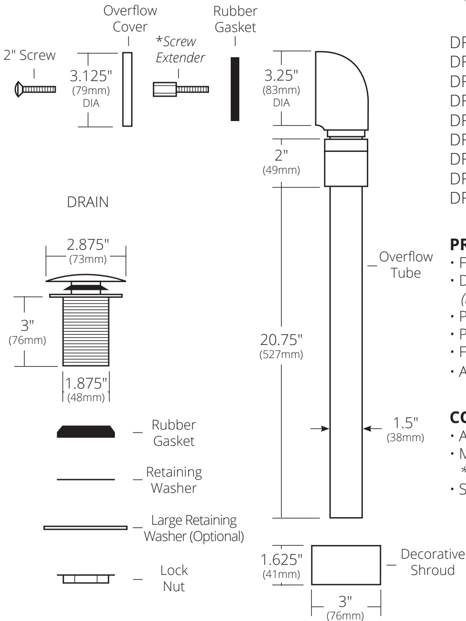
OVERFLOW SIDE VIEW Cover Assembly
