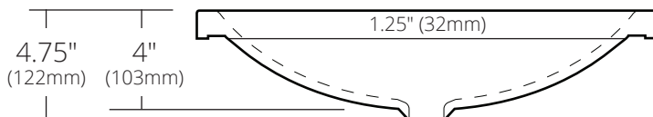
SIDE VIEW
