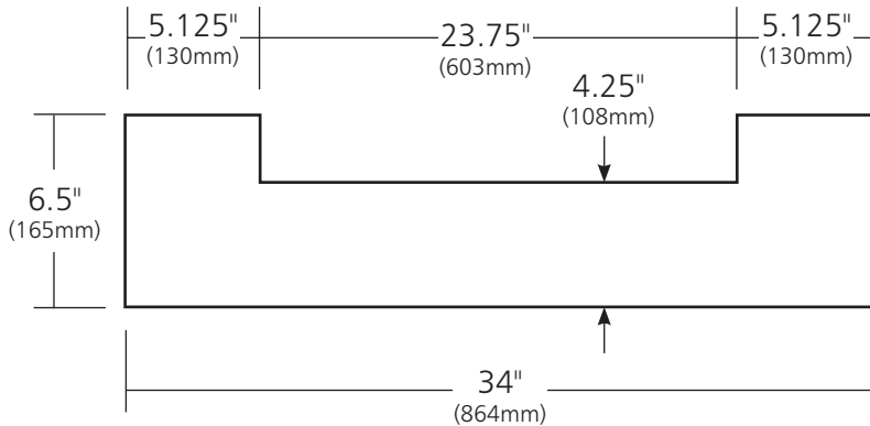
SHELF (optional)
